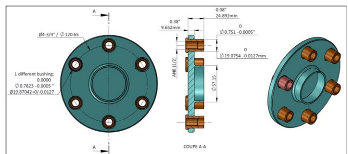
Lycoming O-360-A3A engine prop-shaft, type SAE 2
