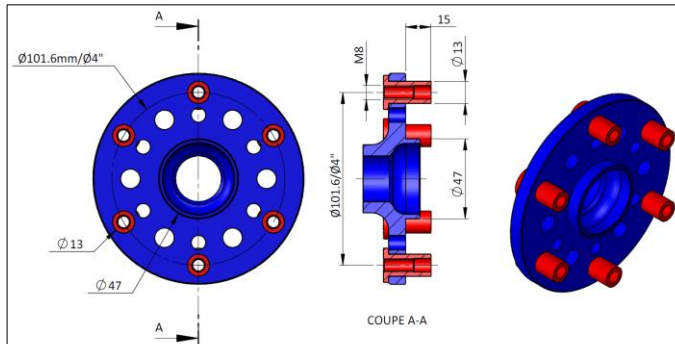
ROTAX 912S engine propeller-shaft
