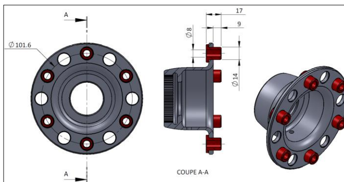
UL Power engine propeller-shaft
