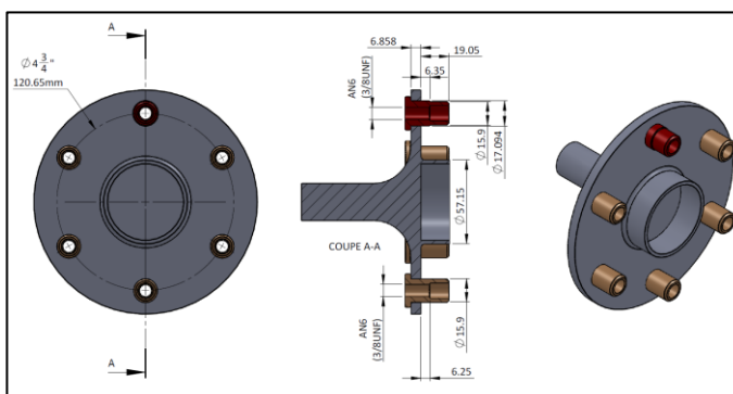
Lycoming O-320-A2A engine prop-shaft, type SAE 2
